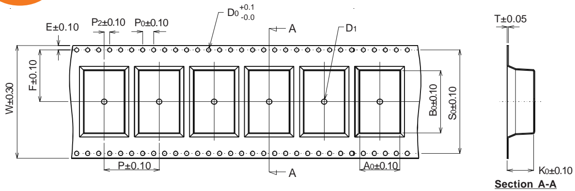
Dimensions for Carrier Tape (Unit : mm)
